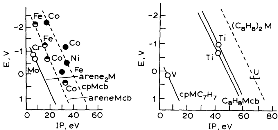
Fig. 4. Dependence of E^0 values on \text{IP}_j for the d^{x/x+1} redox transitions in the series of homo- and heteroligand sandwich complexes: (\text{arene})_2\text{M} , (\text{arene})\text{MCp} , \text{CpMCb} , \text{CpM}(\text{C}_7\text{H}_7) , (\text{COT})\text{MCb} , (\text{COT})_2\text{M} . The dependences calculated from the a_i values found previously are shown by broken lines. (From refs. 32, 33, and 137.)
