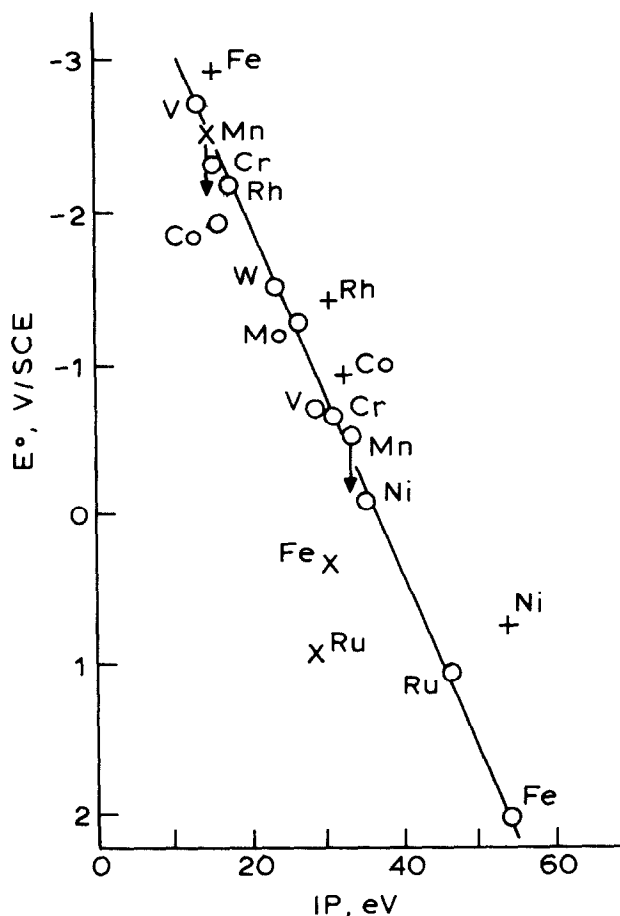
Fig. 2. Dependence of E^0 values for the d^{x/x-1} transitions in the series of metallocenes on the corresponding ionization potentials of the metal. The E^0 values for Cp_2^*Mn are quoted in the case of manganocene; the arrows indicate the shift of E^0 values taking into account the effects of the substituents. (From refs. 32, 33 and 137.)
