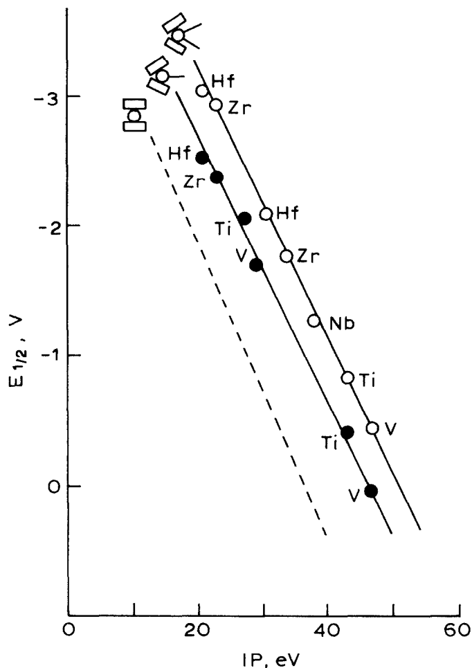
Fig. 5. Linear dependences of the half-wave potentials of the complexes \text{Cp}_2\text{MCl}_2 (○) \text{Cp}_2\text{MCl} (●), and \text{Cp}_2\text{M} (broken line) with the ionization potentials of the corresponding metals. (From refs. 33, 137, and 140(c).)
