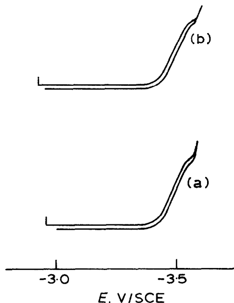
Fig. 1. Steady-state voltammograms of (a) \text{Cp}_2\text{Ru} and (b) \text{Cp}_2\text{Os} in THF/0.04 M \text{Bu}_4\text{NPF}_6 at a microdisc platinum electrode ( r_0 = 20 \mu\text{m} ) at -60^\circ\text{C} (according to Kukharensko et al. [56]).
